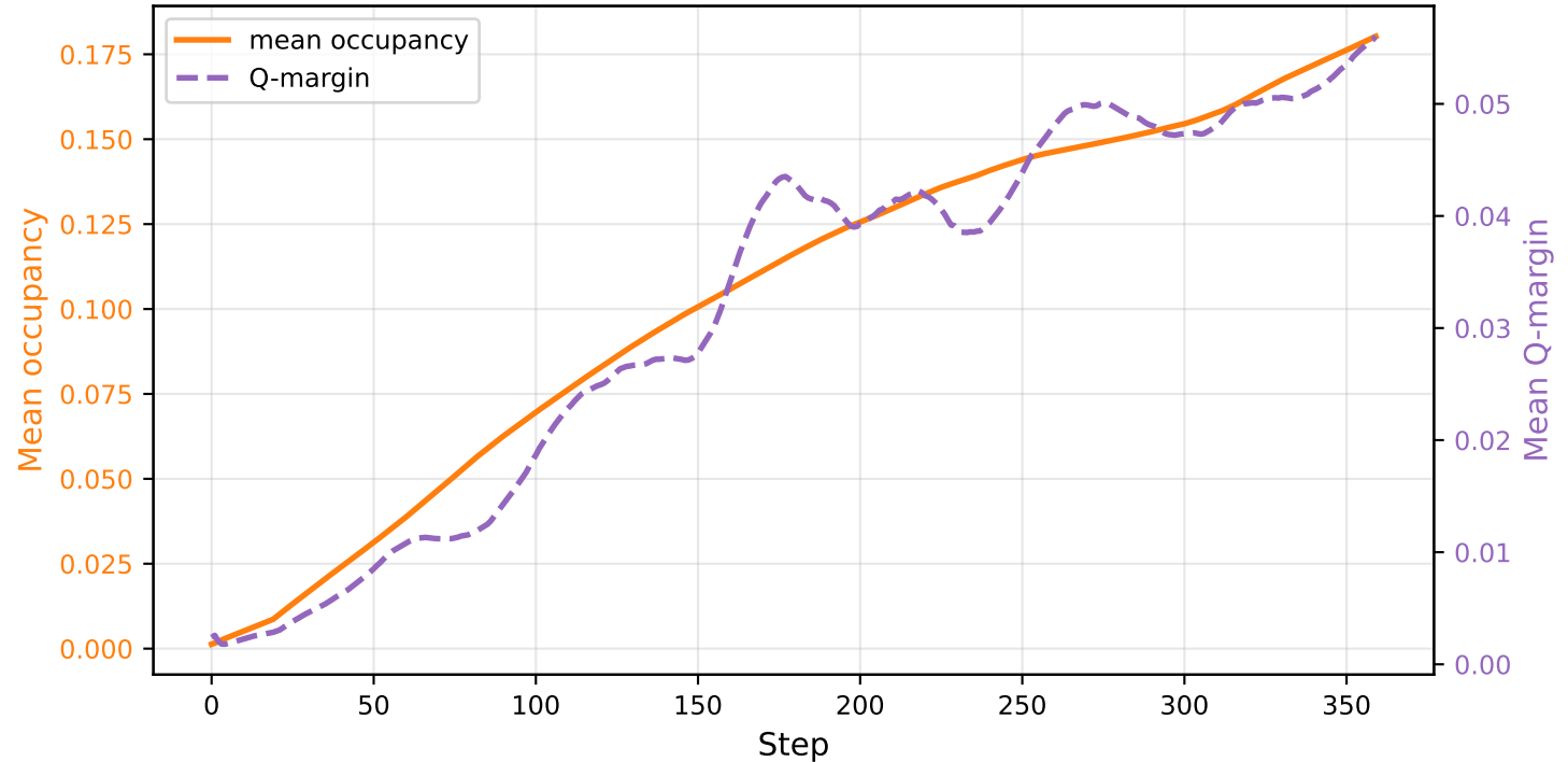
Occupancy and Confidence Margin - LLM_outputs/Jinan/openaigpt-oss-120b/safegat_cityflow_live_output
