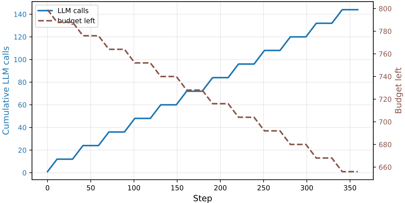
LLM Calls and Budget - LLM_outputs/jinan/openaigpt-oss-120b/safegat_cityflow_live_output
