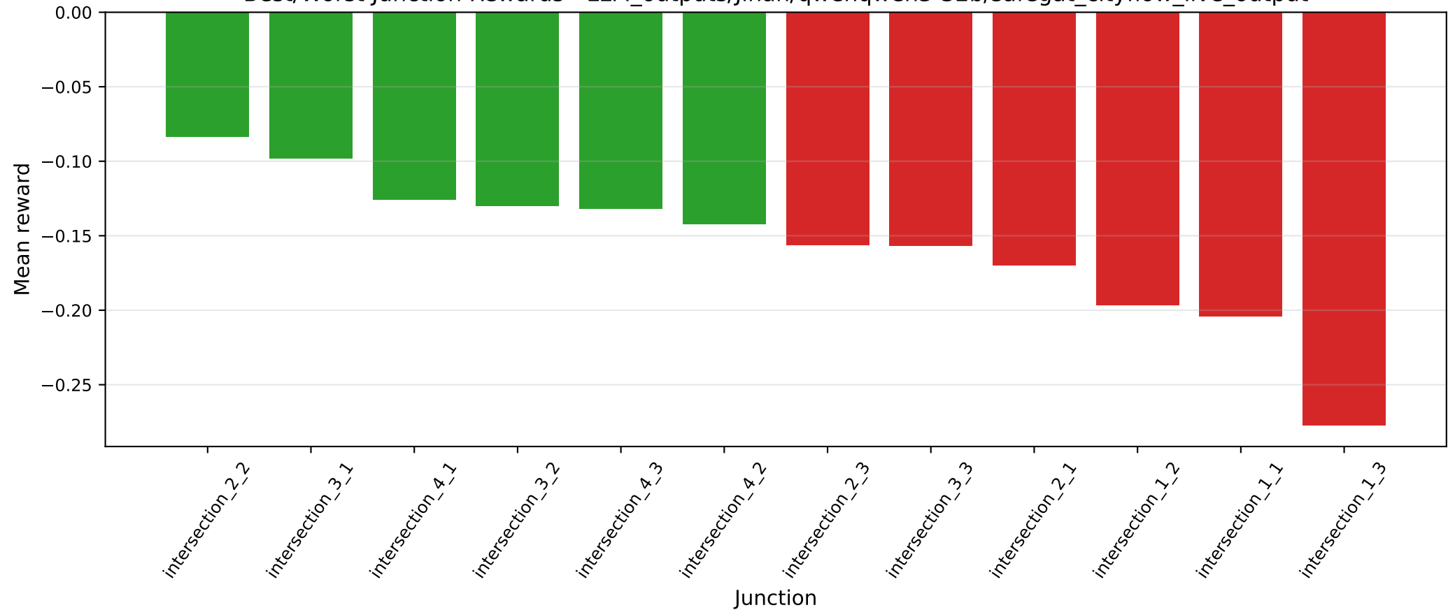
Best/Worst Junction Rewards - LLM_outputs/jinan/qwenqwen3-32b/safegat_cityflow_live_output
