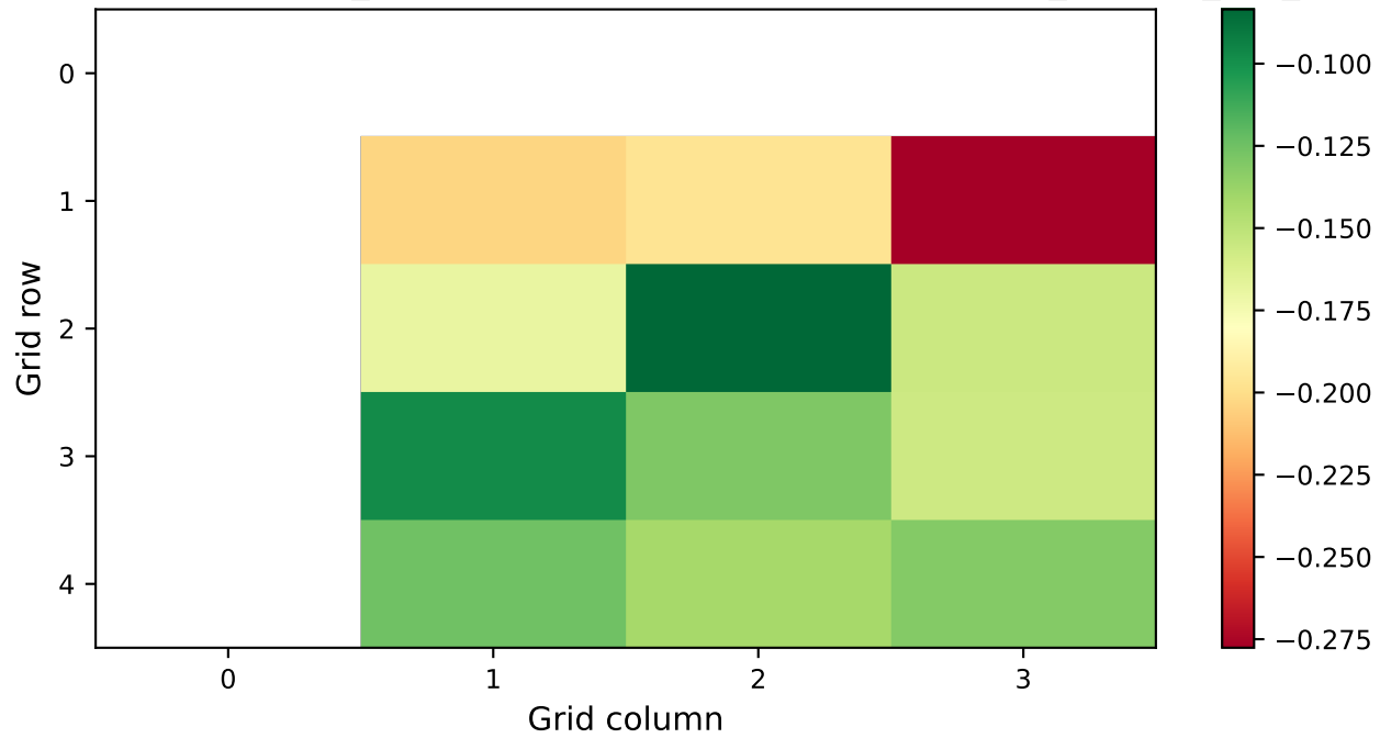
mean_reward Heatmap - LLM_outputs/Jinan/qwenqwen3-32b/safegat_cityflow_live_output
