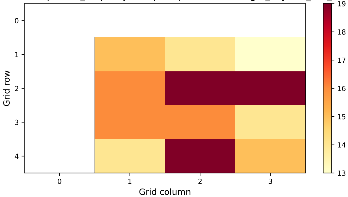
llm_calls Heatmap - LLM_outputs/Jinan/qwenqwen3-32b/safegat_cityflow_live_output
