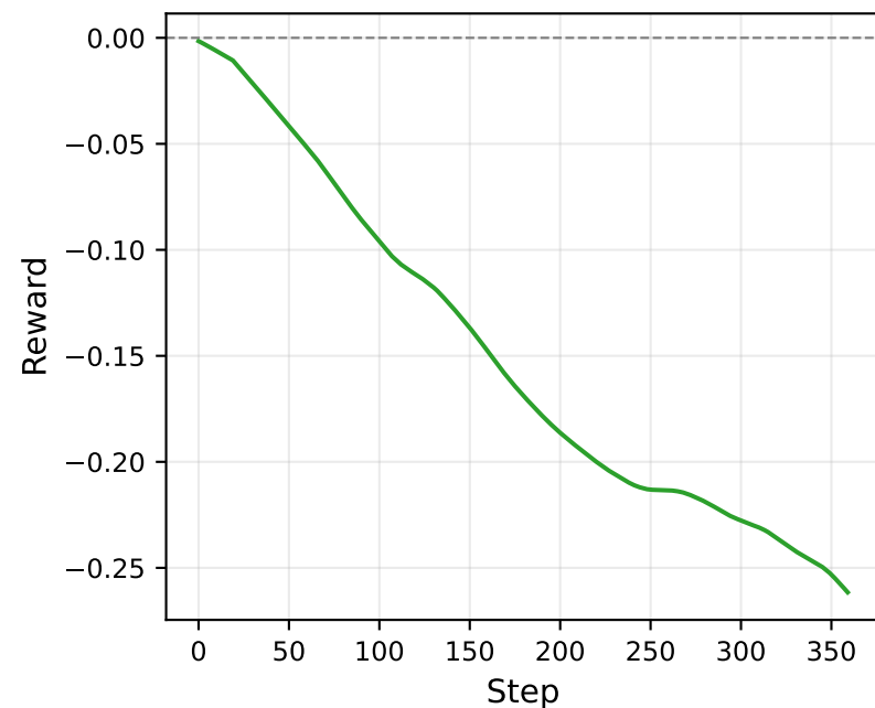
Mean reward
