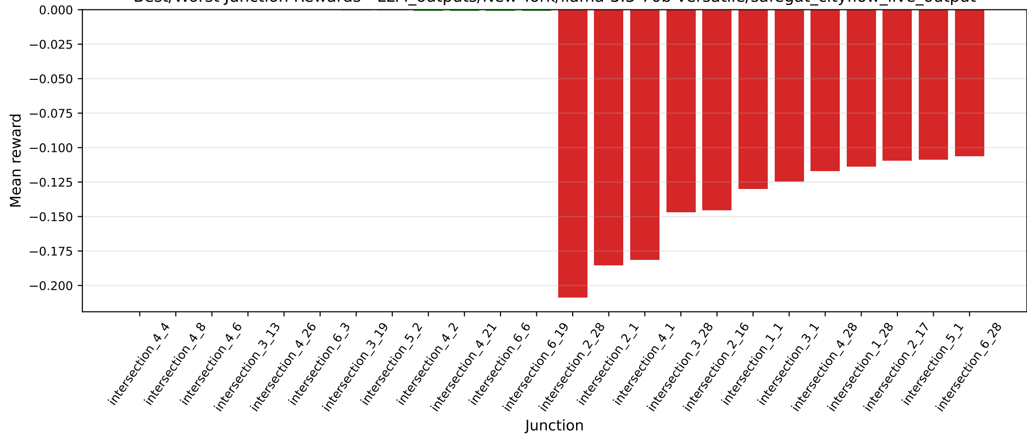
Best/Worst Junction Rewards - LLM_outputs/New York/llama-3.3-70b-versatile/safegat_cityflow_live_output
