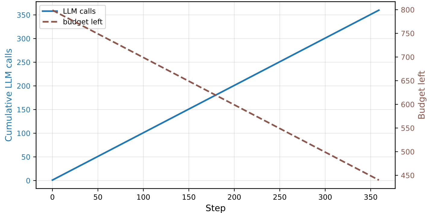
LLM Calls and Budget - LLM_outputs/New York/llama-3.3-70b-versatile/safegat_cityflow_live_output
