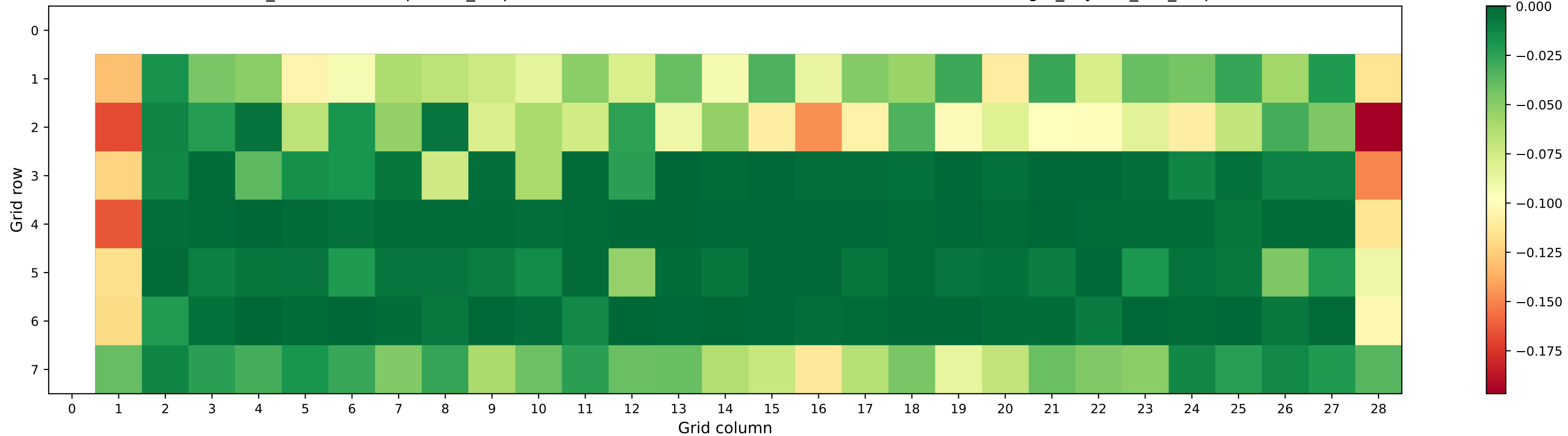
mean_reward Heatmap - LLM_outputs/New York/meta-llamallama-4-scout-17b-16e-instruct/safegat_cityflow_live_output
