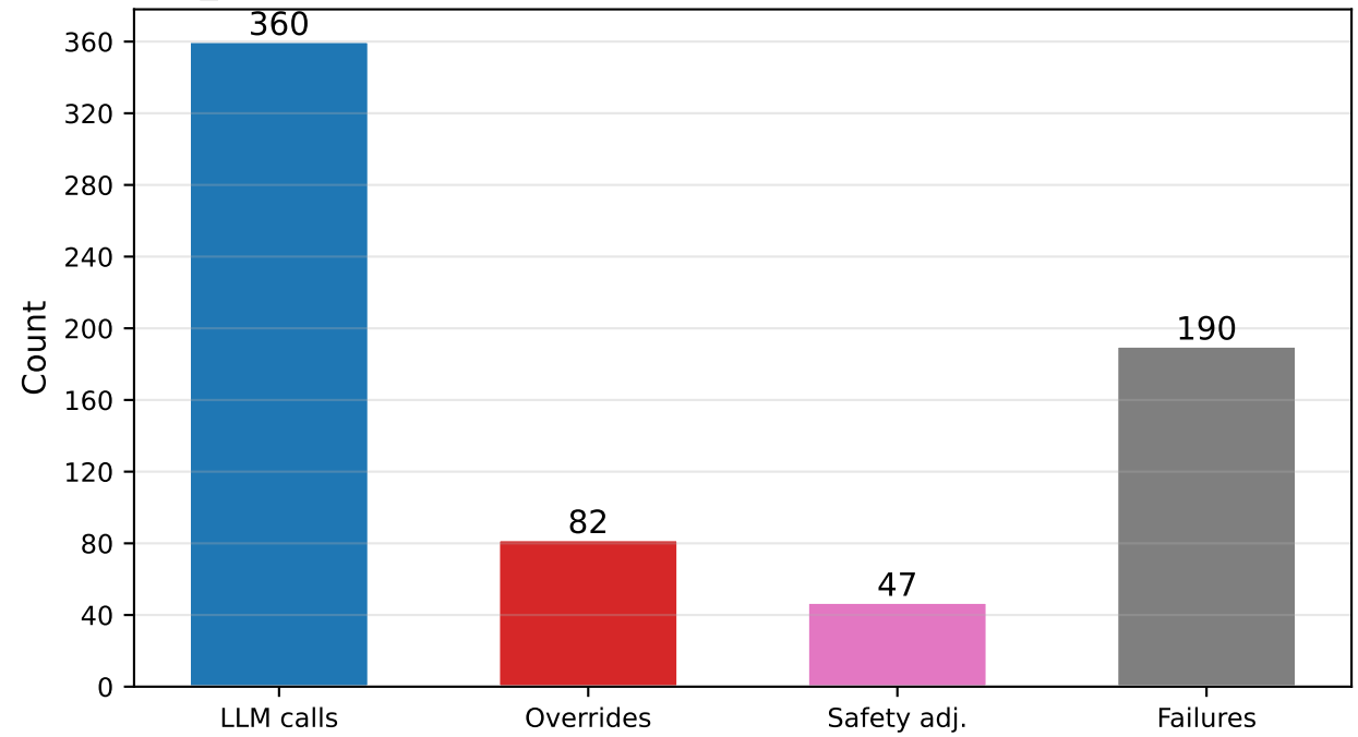
Intervention Summary - LLM_outputs/New York/meta-llamallama-4-scout-17b-16e-instruct/safegat_cityflow_live_output
