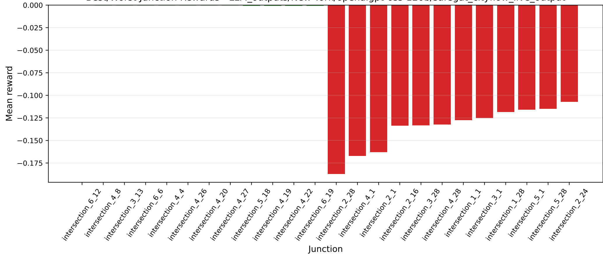
Best/Worst Junction Rewards - LLM_outputs/New York/openaigpt-oss-120b/safegat_cityflow_live_output
