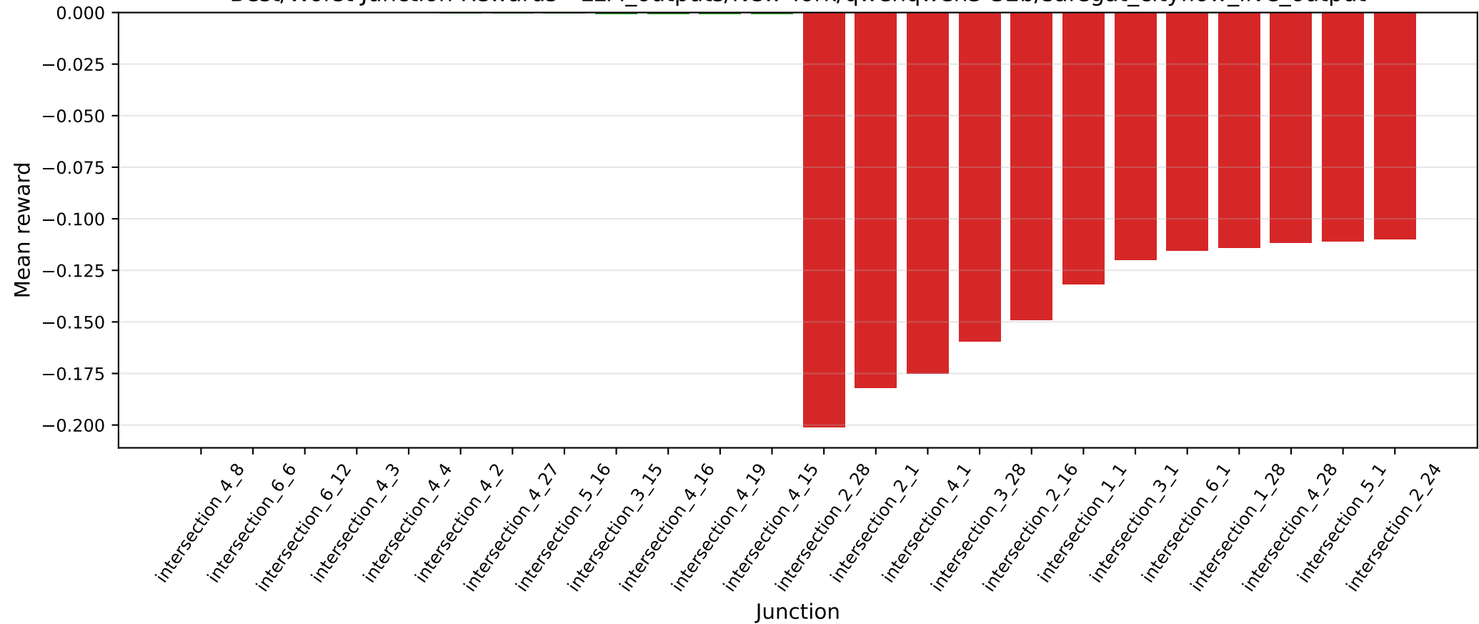
Best/Worst Junction Rewards - LLM_outputs/New York/qwenqwen3-32b/safegat_cityflow_live_output
