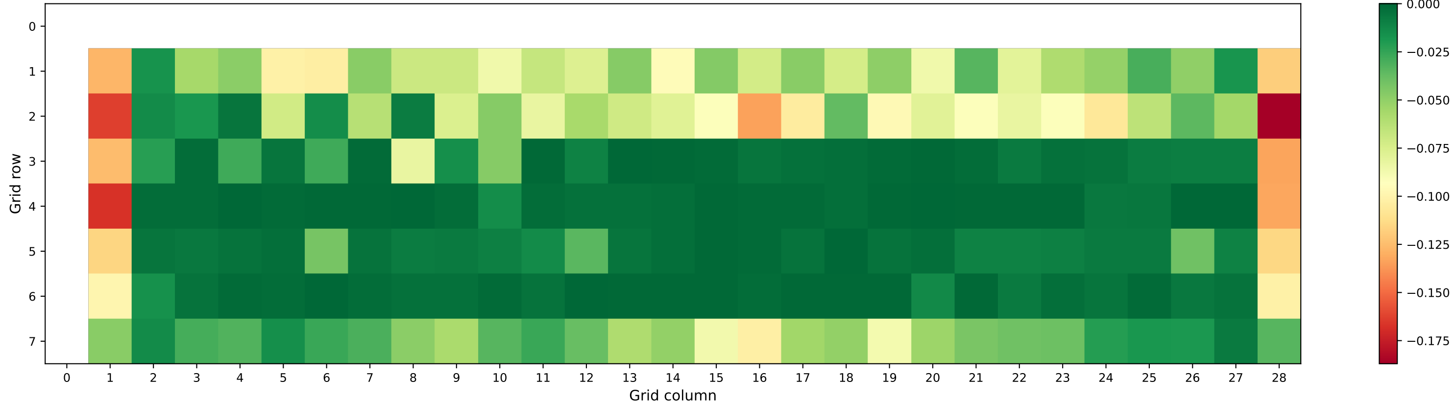
mean_reward Heatmap - NewYork/28_7/safegat_cityflow_live_output
