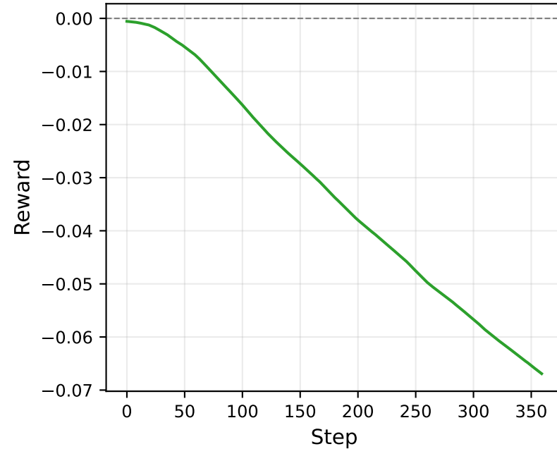
Mean reward
