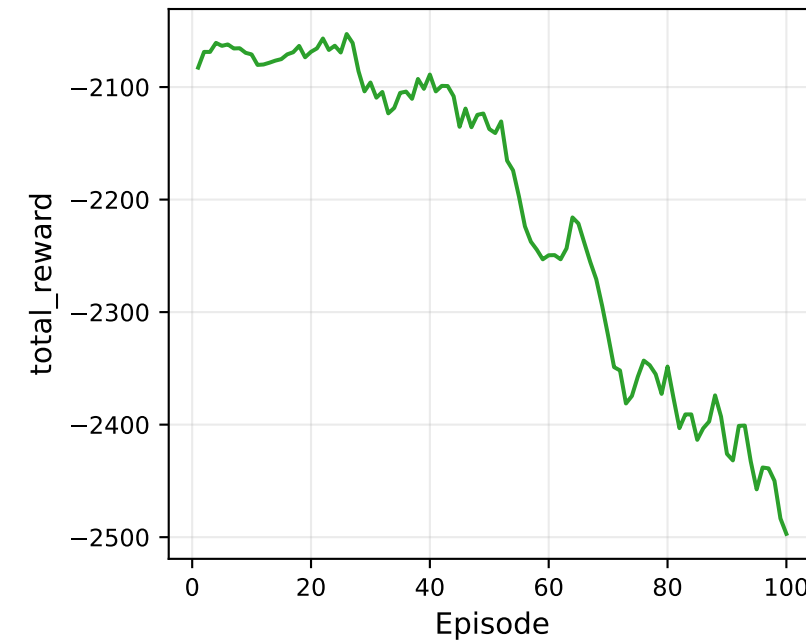
Training reward
