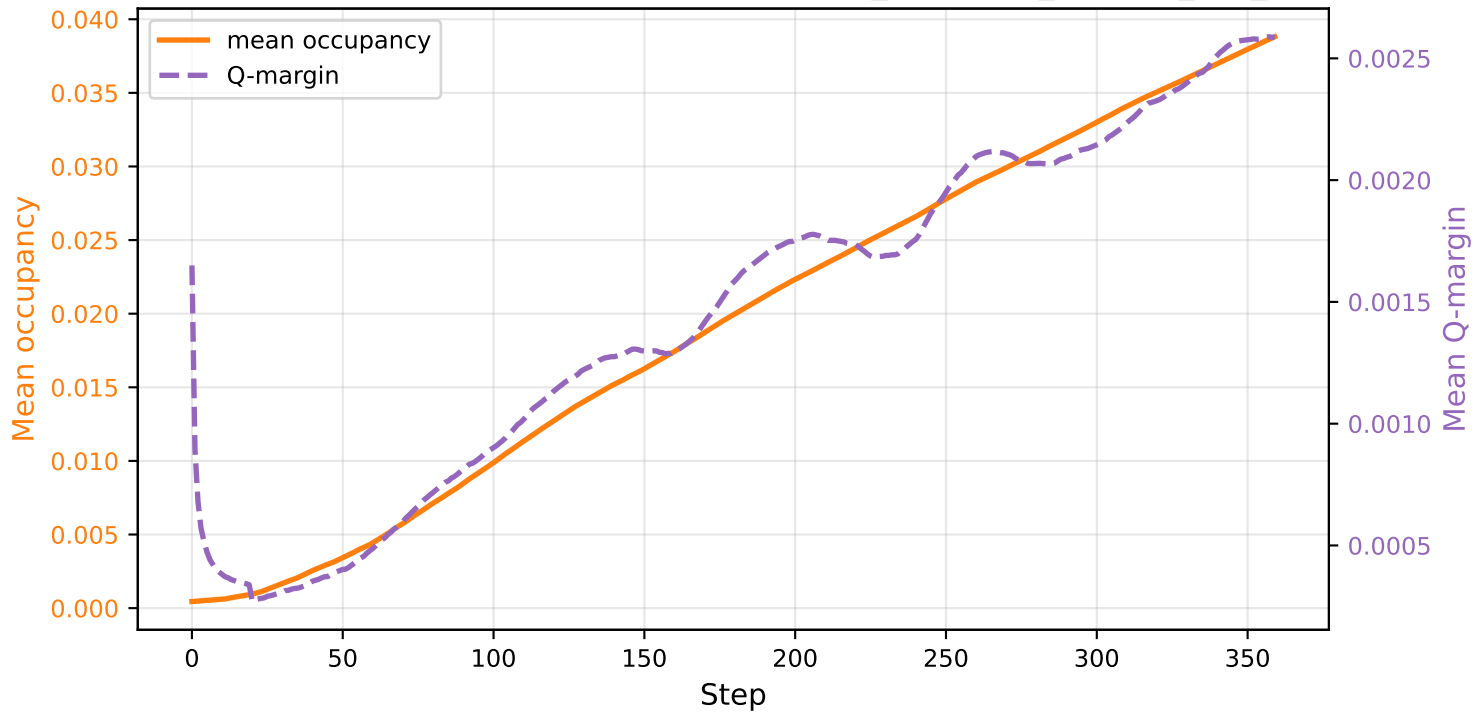
Occupancy and Confidence Margin - NewYork/28_7/safegat_cityflow_live_output
