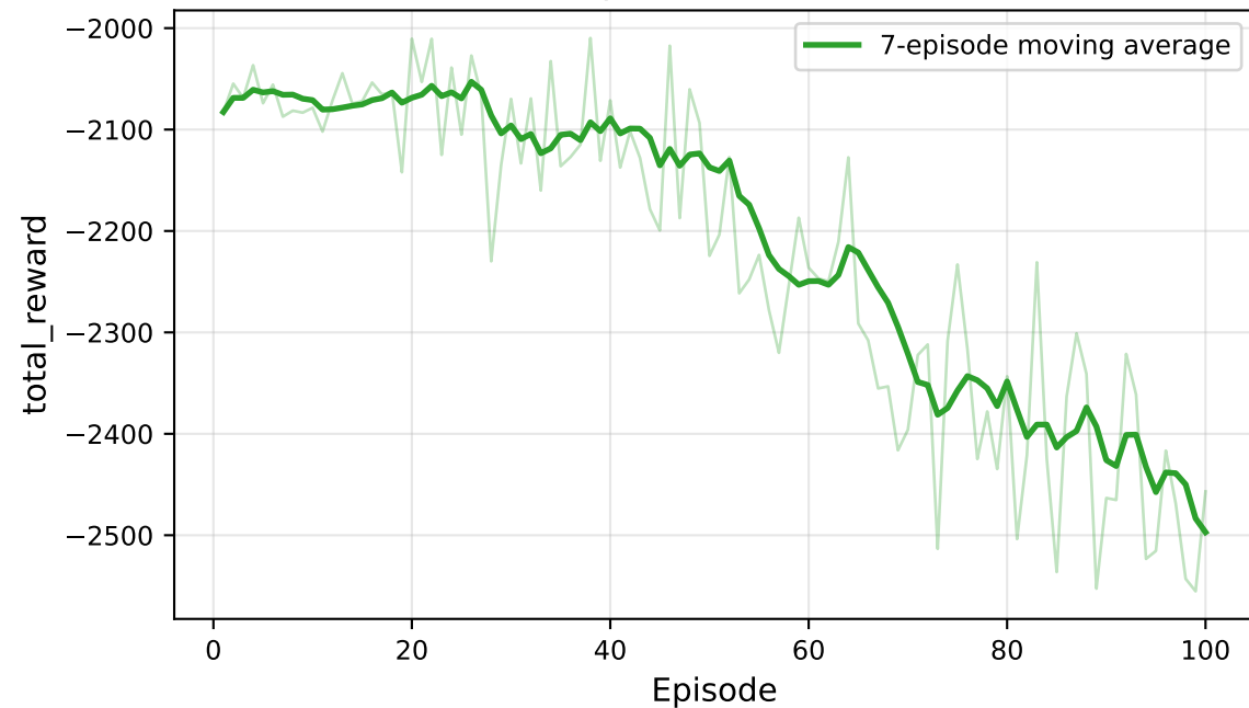
Episode reward
