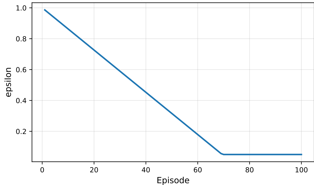
Epsilon schedule
