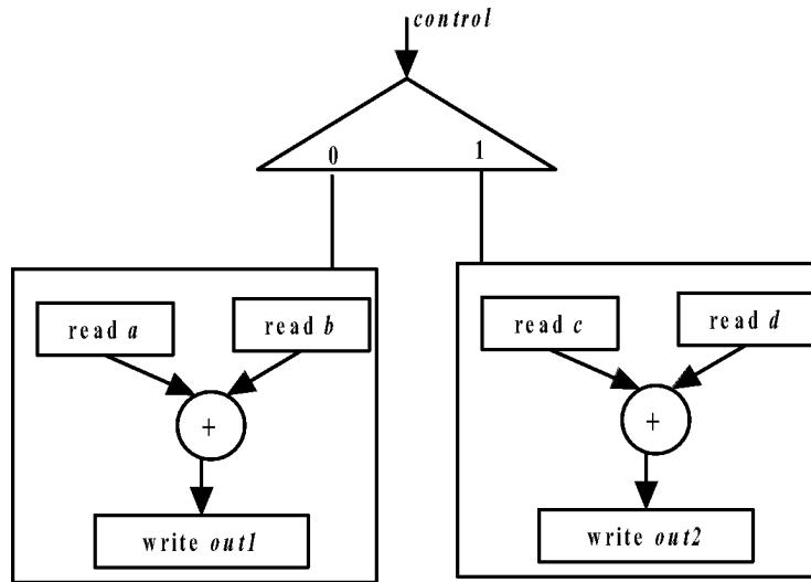
Figure 6. CDFG of the RTL circuit of Figure 5
