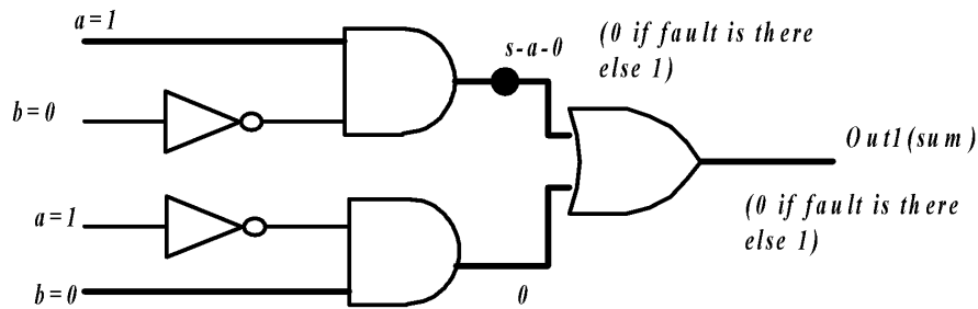
Figure 9. Detection of s-a-0 fault in the circuit for “ Out1(sum) ”
