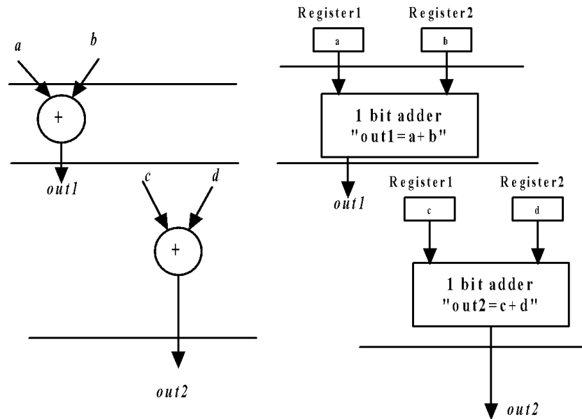
Figure 3. Allocation of operators and variables to hardware units ( 1 adder + 2 Registers)
