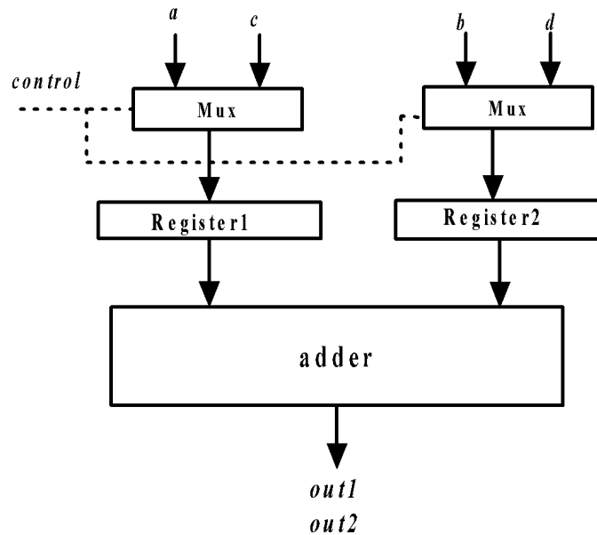
Figure 5. Block diagram with control modules added after allocation and binding
