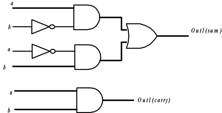
Figure 8. Circuit after logic synthesis for the adder block (of Figure 5)
