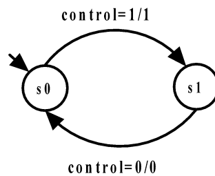
Figure 7. FSM for the control logic of RTL circuit shown in Figure 5
