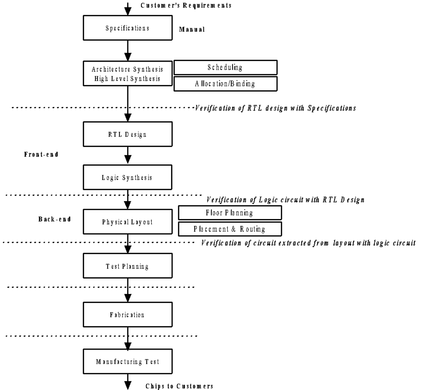
Figure 1. VLSI Design, Verification and Test Flow
