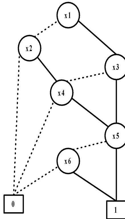
Figure 8. ROBDD of function f with variable ordering [x_1, x_2, x_3, x_4, x_5, x_6]
