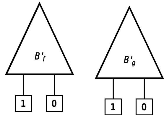
Complement of ROBDDs B_f and B_g
