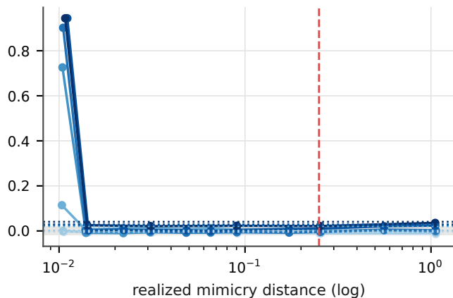
xgboost: FPR increase vs control
