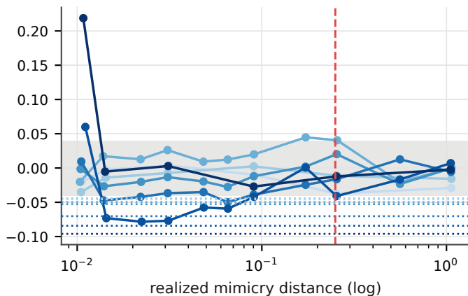
xgboost: TPR drop vs control
