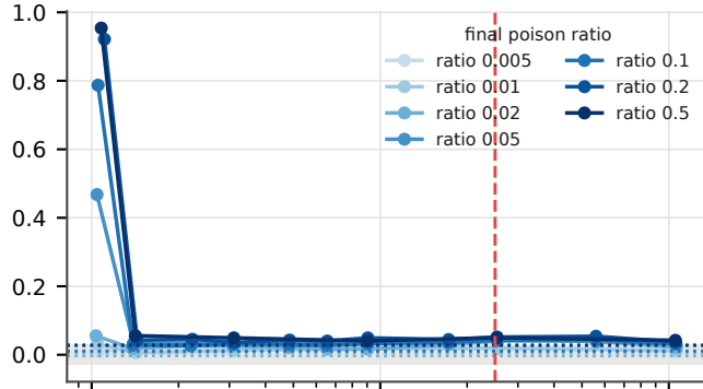
xgboost: FPR increase vs control
