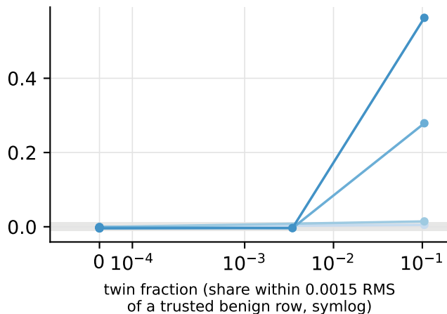
xgboost: FPR increase vs control
