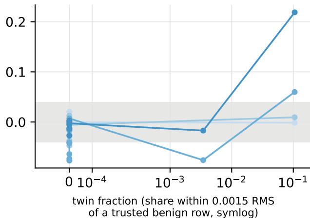
xgboost: TPR drop vs control
