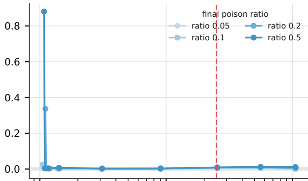
xgboost: FPR increase vs control
