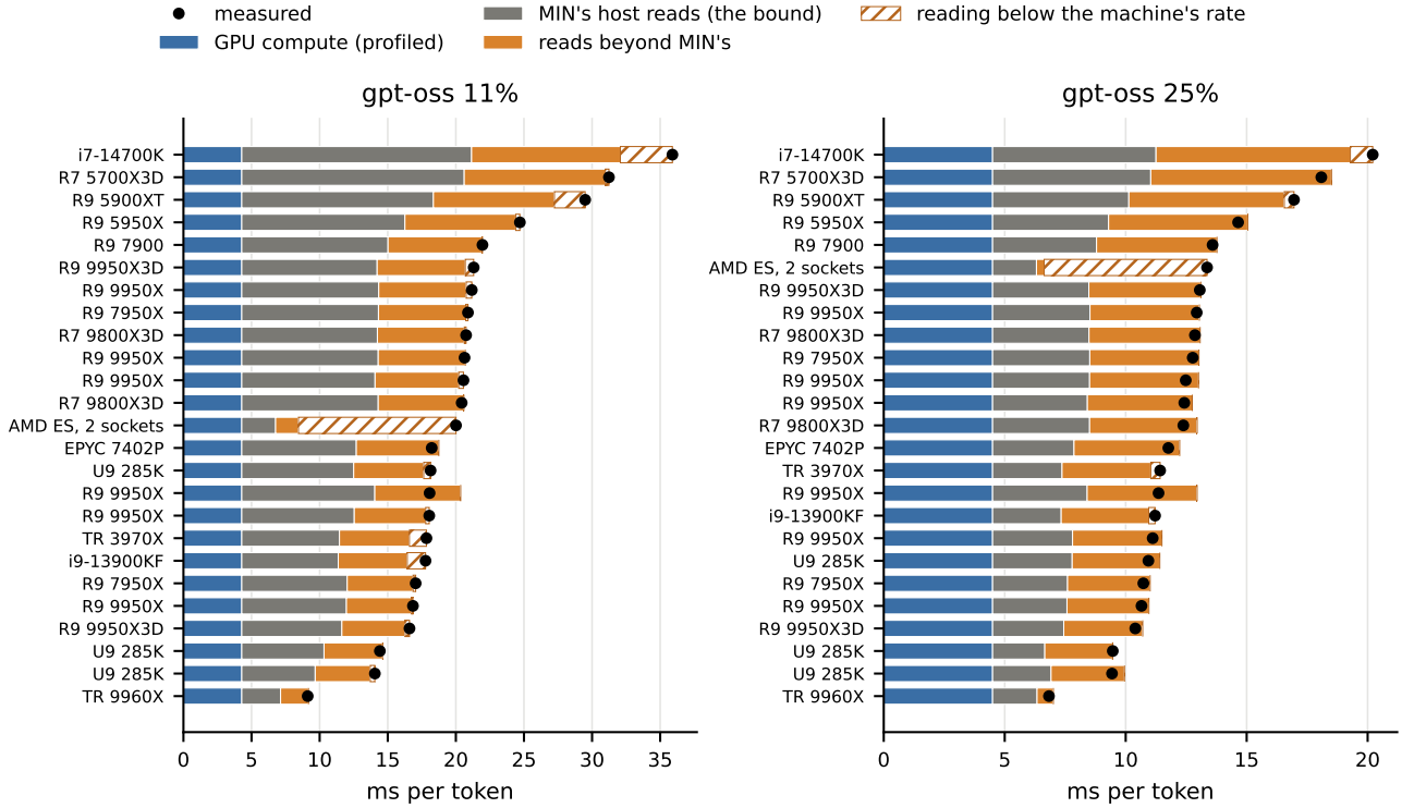
Figure 1. Where the seconds go, machine by machine: the deployed cache’s time per token at the two host-bound gpt-oss budgets split by Eq. (3) into the GPU’s own compute (the median of the profiles at that budget), MIN’s host reads at the machine’s best rate (the bound of Eq. (1)) and the reads the cache makes beyond MIN’s; the dot is the measured time; hatched, the measured time beyond Eq. (3), reading below the machine’s best rate. One launch per machine that ran stably: 24 desktop-class machines and 1 server (AMD ES). Nothing is fitted: G comes from profiles, the reads from the engine’s counters and the rate from each machine’s probe.
