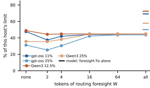
Figure 8. The first oracle job (093, host O1): speed as a percentage of this host’s limit against the window W of future routing the hit-optimal oracle sees, at the four host-bound cells. “none” is the online policy; “all” the whole sequence; points are connected for the trend only. The tick at the right is the model’s foresight-only term for the cell, the speed it predicts with that one fix; the oracle’s host traffic sits at 89–94% of the probe’s best rate at every window, so its speed is R^* over its reads times that utilisation, 44–45% of the limit with the whole sequence in view.
