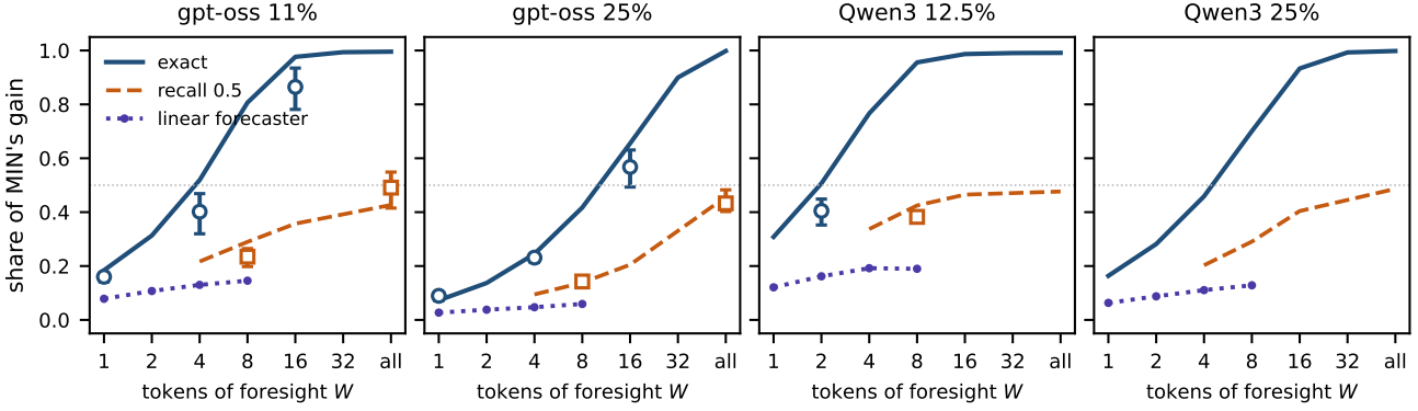
Figure 4. The value of partial foresight at the four host-bound budgets: the share of MIN’s gain over admit every miss recovered by exact routing of the next W tokens (solid), by a window whose experts are each right with probability 0.5 (dashed), and by a linear forecaster fitted on other text (dotted), in host reads on the AIME routing the engine runs; markers: the same share in time per token on the panel hosts (mean, and range over hosts; 10 hosts for gpt-oss, 3 for Qwen3 at 12.5%; no Qwen3 run at 25%). The grey line marks half of the gain.
