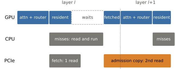
Figure 1. One decode step of the deployed cache, schematically. Blue: the GPU’s own kernels, whose time per token is G . Grey: host reads of the misses, which the step waits for. Orange: the background copy that fills an admitted expert’s slot, a second read that overlaps the next layer.
