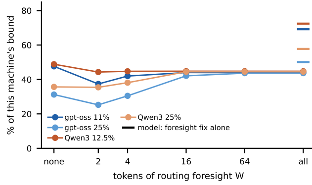
Fig. 6. The first oracle job (093, host O1): speed as a percentage of this machine’s bound against the window W of future routing Belady-2R sees, at the four host-bound cells. “none” is the deployed cache; “all” the whole sequence; points are connected for the trend only. The tick at the right is the model’s foresight-only term for the cell, the speed it predicts with that one fix; the oracle’s host traffic sits at 89–94% of the probe’s best rate at every window, so its speed is R^* over its reads times that utilisation, 44–45% of the bound with the whole sequence in view.
