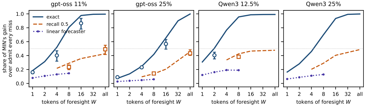
Fig. 5. Baseline here: admit every miss , not the deployed cache. The value of partial foresight at the four host-bound budgets: the share of MIN’s gain over admitting every miss recovered by exact routing of the next W tokens (solid), by a window whose experts are each right with probability 0.5 (dashed), and by a linear forecaster fitted on other text (dotted), in host reads on the routing the engine runs. Markers: the same share in time per token on the panel machines (mean and range over machines; 10 machines for gpt-oss, 3 for Qwen3 at 12.5%). The grey line marks half of the gain.
