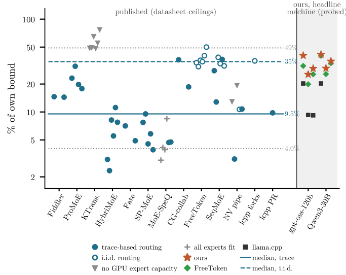
Fig. 9. Published MoE-offloading measurements (52 rows from 13 sources) as a percentage of their own bound, computed from the paper’s hardware at datasheet rates and, where a routing trace of the model exists, the per-layer Belady optimum (filled); hollow points assume uniform routing, which overstates the optimum’s reads and so the percentage; the dotted lines are the class medians (no GPU expert capacity, 49.0%; every expert resident, 4.0%). Right: our cache, FreeToken and stock llama.cpp on host B against the probed per-layer bound of Table III (the pooled bound FreeToken’s and llama.cpp’s designs allow is 0–10% higher).
