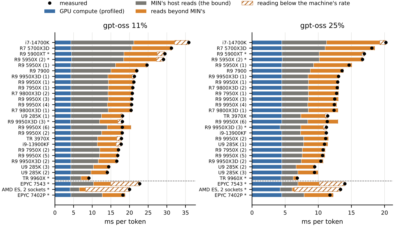
Fig. 7. The split implied by Eq. (4) (exploratory): the deployed cache’s time per token at the two host-bound gpt-oss budgets, machine by machine, split into the GPU’s compute ( G , profiled on the machine, or the median profile where none was taken or it captured no decode kernels), MIN’s host reads at the machine’s best rate (the bound of Eq. (1)) and the reads the cache makes beyond MIN’s. The dot is the measured time; hatched, the measured time beyond Eq. (4), reading below the machine’s best rate; a bar that ends past the dot is an over-prediction. Machines with the same processor are numbered in order of rental. One launch per machine that ran stably: 25 with consumer processors (above the dashed line) and 3 with server processors (below). *: first rented for a registered test of Eq. (4).
