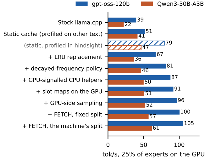
Fig. 8. Ablation at 25% of experts on the GPU (15 AIME-25 problems, 256 tokens, host A). Each step adds one component to the one above; the hatched row is not a step: a static cache of each layer’s 32 most requested experts counted on the measured problems themselves.
