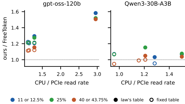
Figure 3: Ours over FreeToken’s better backend in every same-machine comparison of the current engine (jobs 076–088), against the machine’s CPU-to-PCIe read ratio (FreeToken’s own probe). Filled: FETCH table from the law on that machine; hollow: the fixed table. The rightmost gpt-oss points are the Core i9-14900K with FreeToken’s executor on its performance cores (job 088; the confounded job 085 points are omitted); the rightmost Qwen3 points are the Ryzen 9 7900.
