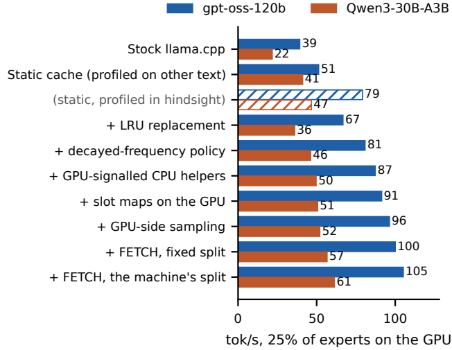
Fig. S3. Ablation at 25% of experts on the GPU (15 AIME-25 problems, 256 tokens, host A). Each step adds one component to the one above; the hatched row is not a step: a static cache of each layer’s 32 most requested experts counted on the measured problems themselves.
