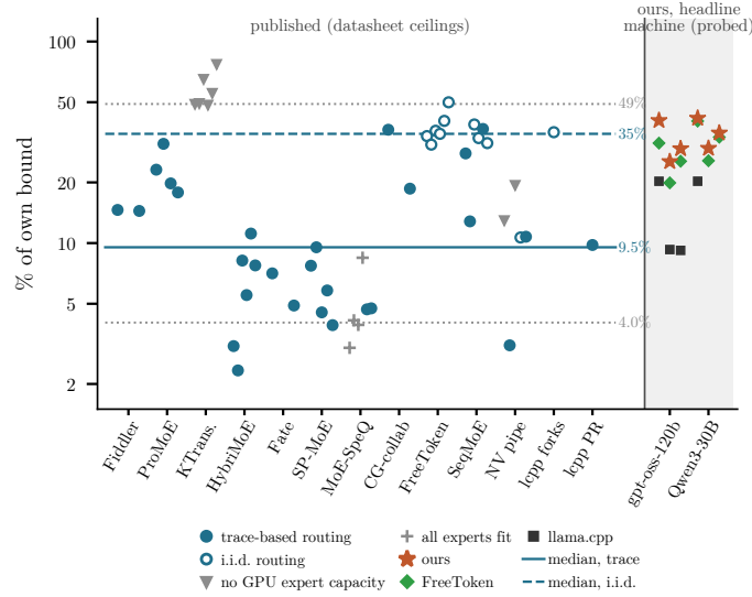
Fig. S4. Published MoE-offloading measurements (52 rows from 13 sources) as a percentage of their own bound, computed from the paper’s hardware at datasheet rates and, where a routing trace of the model exists, the per-layer Belady optimum (filled); hollow points assume uniform routing, which overstates the optimum’s reads and so the percentage; the dotted lines are the class medians (no GPU expert capacity, 49.0%; every expert resident, 4.0%). Right: our cache, FreeToken and stock llama.cpp on host B against the probed per-layer bound of Table III (the pooled bound FreeToken’s and llama.cpp’s designs allow is 0–10% higher).
