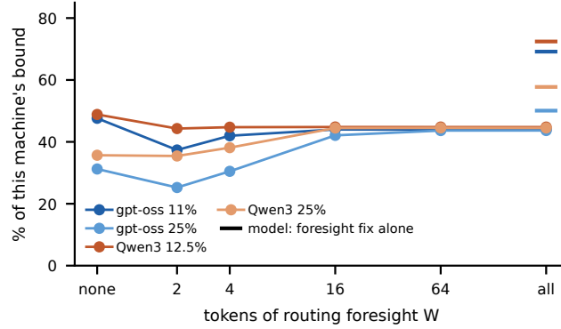
Fig. S1. The first oracle job (093, host O1): speed as a percentage of this machine’s bound against the window W of future routing Belady-2R sees, at the four host-bound cells. “none” is the deployed cache; “all” the whole sequence; points are connected for the trend only. The tick at the right is the model’s foresight-only term for the cell, the speed it predicts with that one fix; the oracle’s host traffic sits at 89–94% of the probe’s best rate at every window, so its speed is R^* over its reads times that utilisation, 44–45% of the bound with the whole sequence in view.
