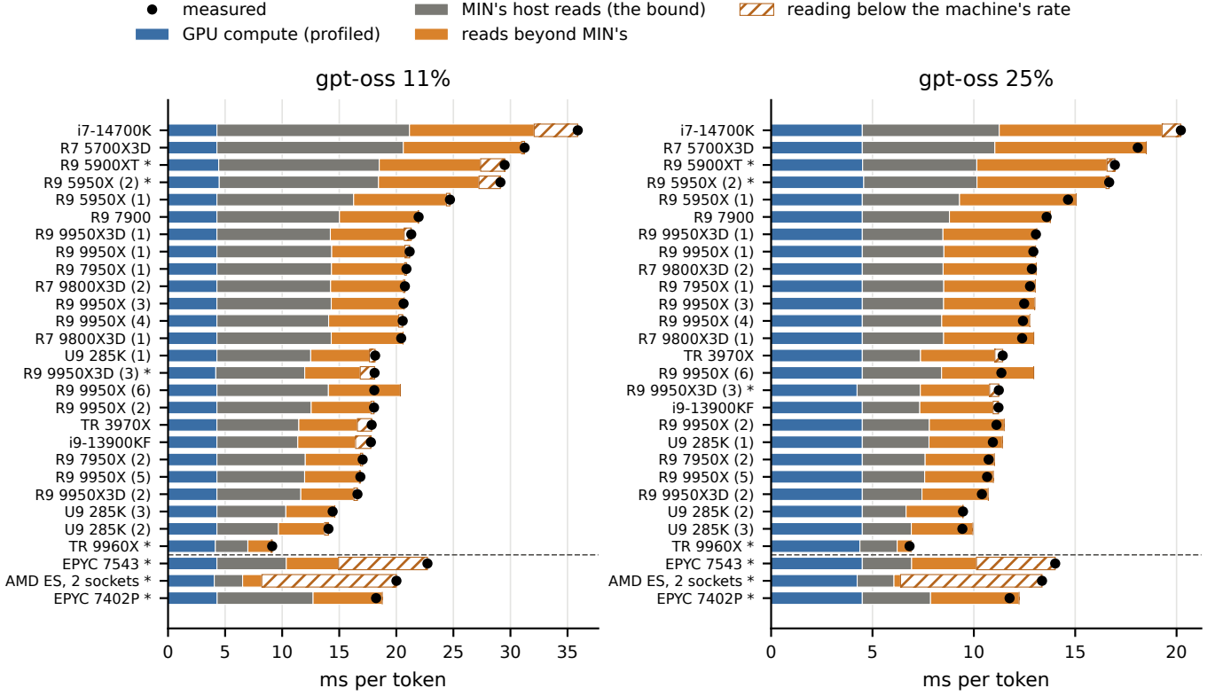
Fig. S2. The split implied by Eq. (S1) (exploratory): the deployed cache’s time per token at the two host-bound gpt-oss budgets, machine by machine, split into the GPU’s compute ( G , profiled on the machine, or the median profile where none was taken or it captured no decode kernels), MIN’s host reads at the machine’s best rate (the bound of Eq. (1)) and the reads the cache makes beyond MIN’s. The dot is the measured time; hatched, the measured time beyond Eq. (S1), reading below the machine’s best rate; a bar that ends past the dot is an over-prediction. Machines with the same processor are numbered in order of rental. One launch per machine that ran stably: 25 with consumer processors (above the dashed line) and 3 with server processors (below). *: first rented for a registered test of Eq. (S1).
