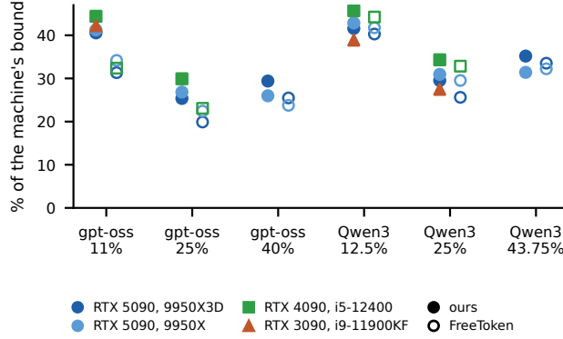
Figure 1: Ours (filled) and FreeToken (hollow) as a percentage of each machine’s own bound (exact optimum, the machine’s highest probed host rate, the card’s datasheet rate) at every cell of Table 3: two RTX 5090 machines, an RTX 4090 and an RTX 3090 (FreeToken’s 3090 cells, its carried-over backend running below llama.cpp, are omitted). The bound ranges from 41 to 519 tok/s across these cells; ours stays at 25–46% of it.
