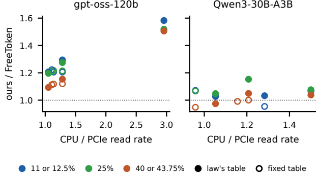
Figure 2: Ours over FreeToken’s better backend (carried over from host B on host S) in every same-machine comparison of the current engine on the two models of Table 3 (eight machines), against the machine’s CPU-to-PCIe read ratio (FreeToken’s own probe). Filled: FETCH table from the model on that machine; hollow: the fixed table. The rightmost gpt-oss points are a Core i9-14900K with FreeToken’s executor on its performance cores; the rightmost Qwen3 points are a Ryzen 9 7900.
