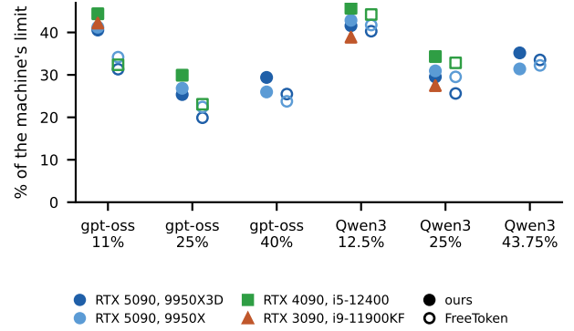
Figure 5: Ours (filled) and FreeToken (hollow) as a percentage of each machine’s own speed limit (exact optimum, the machine’s highest probed host rate, the card’s datasheet rate) at every cell of Table 7: two RTX 5090 hosts, an RTX 4090 and an RTX 3090 (FreeToken’s 3090 cells, its carried-over backend running below llama.cpp, are omitted). The limit ranges from 41 to 519 tok/s across these cells; ours stays at 25–46% of it.
