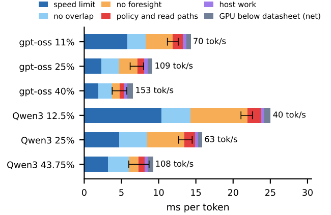
Figure 1: Where the seconds go: Shapley attribution of the gap between our cache’s measured time per token and the speed limit, for every cell of Table 1, averaged over all 120 orders in which the five fixes can be applied. Fixes: overlapping host reads with GPU work, which in Eq. (2)’s form also moves experts onto the CPU until the two paths balance; the optimum’s reads instead of the best online policy’s (foresight); the best online policy’s reads at the probe’s highest rate instead of the engine’s reads through Eq. (1) (policy and read paths); the engine’s per-token host work; and GPU kernels at the datasheet rate, the term that closes the model on the measured time. Whiskers: the range of foresight’s marginal cost over the orders.
