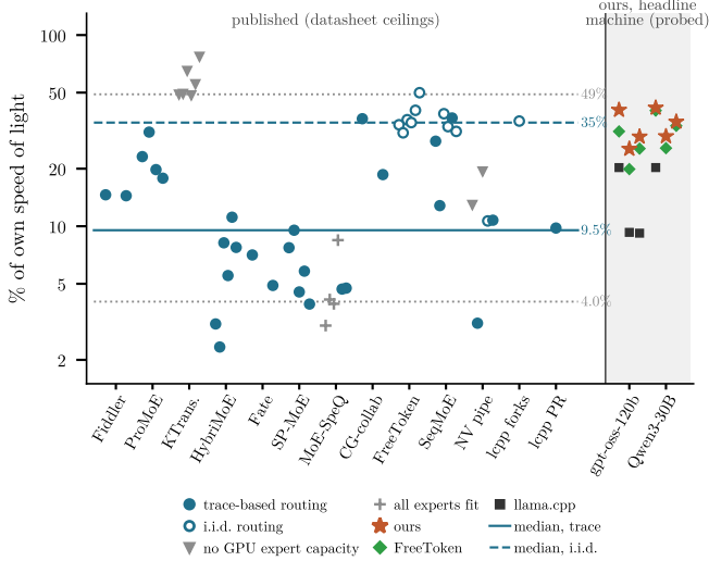
Figure 2: Published MoE-offloading measurements (52 rows from 13 sources) as a percentage of their own speed of light, computed from the paper’s hardware at datasheet rates and, where a routing trace of the model exists, the per-layer Belady optimum (filled); hollow points assume uniform routing, which overstates the optimum’s reads and so the percentage. Right: our cache, FreeToken and stock llama.cpp on listing B against the probed limit of Table 1.
