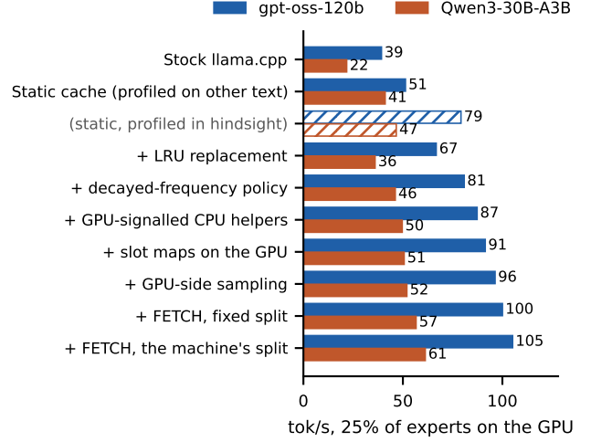
Figure 3: Ablation at 25% of experts on the GPU (15 AIME-25 problems, 256 tokens, listing A). Each step adds one component to the one above; the hatched row is not a step: a static cache of each layer’s 32 most requested experts counted on the measured problems themselves.
