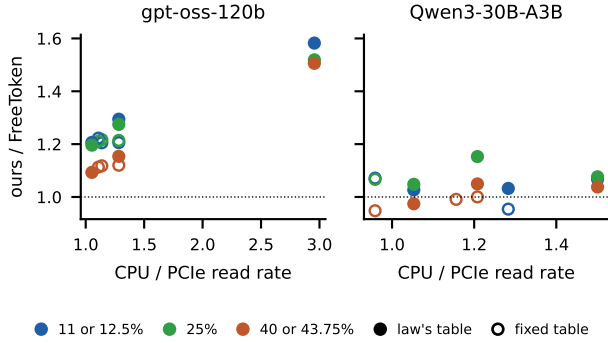
Figure 5: Ours over FreeToken’s better backend (carried over from listing B on the stock-clock host) in every same-machine comparison of the current engine on the two models of Table 1 (eight hosts), against the machine’s CPU-to-PCIe read ratio (FreeToken’s own probe). Filled: FETCH table from the law on that machine; hollow: the fixed table. The rightmost gpt-oss points are a Core i9-14900K with FreeToken’s executor on its performance cores; the rightmost Qwen3 points are a Ryzen 9 7900.
