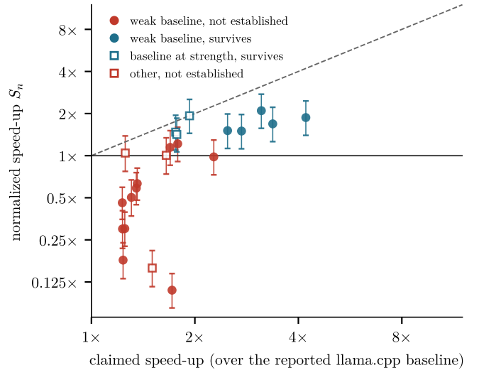
Figure 1: Claimed speed-up (over the row’s strongest reported llama.cpp baseline, else its strongest baseline) against normalised speed-up (over the predicted equal-memory llama.cpp baseline), adjudicated rows, with the band. Below the dashed line the claim shrinks against a strong baseline; below 1 the gain is not established.
