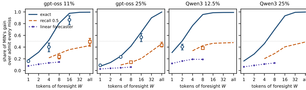
Figure 5. Baseline here: admit every miss , not the deployed cache. The share of MIN’s gain over admitting every miss recovered, in host reads on the routing the engine runs, by exact routing of the next W tokens (solid), by a window whose experts are each right with probability 0.5 (dashed) and by a linear forecaster fitted on other text (dotted). Markers: the same share in time per token (mean and range over the panel’s main-job machines: 10 for gpt-oss, 3 for Qwen3 12.5%). Grey line: half of the gain.
