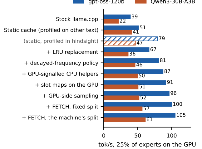
Figure 2: Ablation at 25% of experts on the GPU (15 AIME-25 problems, 256 tokens, one machine; job 087). Each step adds one component to the one above; the hatched row is not a step: a static cache of each layer’s 32 most requested experts counted on the measured problems themselves.
