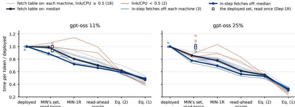
Figure 2. Where the seconds go, measured: each state's time per token relative to the deployed cache on the same machine (lower is faster), as oracles change what is cached (MIN's set, read twice; squares: the deployed set, read once), then both, then when it is read, with the two bounds for reference. One line per machine. Grey and orange: the deployed read path, with the fetch table (orange: link-to-CPU ratio below 0.5). Blue: the registered test with the in-step fetches off (diamonds: the deployed cache without them). Thick lines: medians over the fast-link machines.
