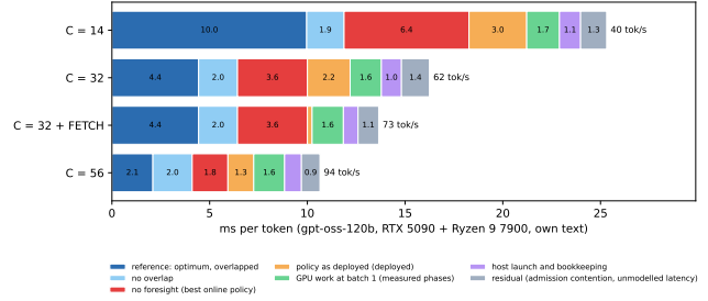
Figure 1: Where the seconds go: gpt-oss-120b, from the speed limit (left) to measured time per token (right), one cause at a time (RTX 5090 + Ryzen 9 7900, own text, job 072). The largest single term at small budgets is foresight, the gap between the optimum and the best online policy; at large budgets it is GPU work at batch 1 and per-token host work.
