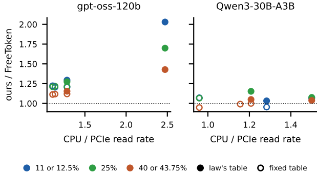
Figure 3: Ours over FreeToken’s better backend in every same-machine comparison of the current engine (jobs 076–085b), against the machine’s CPU-to-PCIe read ratio (FreeToken’s own probe). Filled: FETCH table from the law on that machine; hollow: the fixed table. The rightmost gpt-oss points are the Core i9-14900K, where FreeToken’s CPU backend failed (Section 5); the rightmost Qwen3 points are the Ryzen 9 7900.
