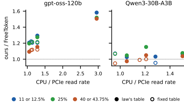
Figure 4: Ours over FreeToken’s better backend (carried over from host B on host S) in every same-machine comparison of the current engine on the two models of Table 2 (eight hosts), against the machine’s CPU-to-PCIe read ratio (FreeToken’s own probe). Filled: FETCH table from the model on that machine; hollow: the fixed table. The rightmost gpt-oss points are a Core i9-14900K with FreeToken’s executor on its performance cores; the rightmost Qwen3 points are a Ryzen 9 7900.
