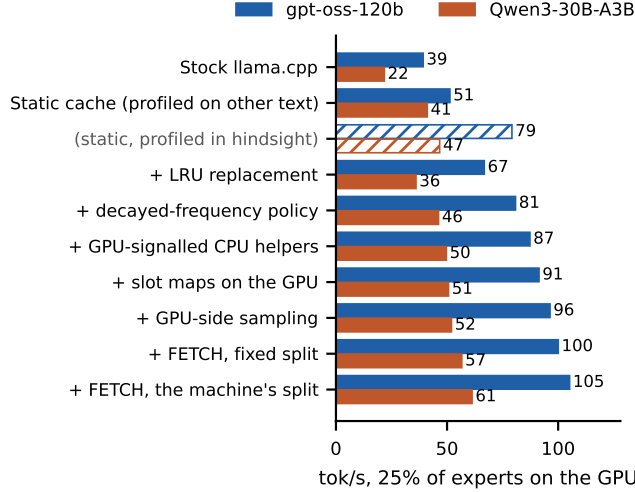
Figure 7: Ablation at 25% of experts on the GPU (15 AIME-25 problems, 256 tokens, host A). Each step adds one component to the one above; the hatched row is not a step: a static cache of each layer’s 32 most requested experts counted on the measured problems themselves.
