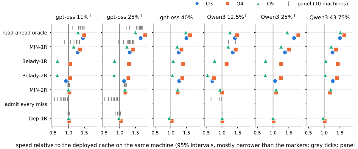
Figure 3. What foresight is worth, by how it is spent: speed of each configuration of Table 2 relative to the deployed cache on the same machine, at the six budgets ( † host-bound). Three machines at every budget (O3–O5: two Ryzen 9 9950X and a 9950X3D); the 10 panel machines (grey ticks) at the two host-bound gpt-oss budgets, and 3 of them at Qwen3 12.5%. MIN-1R gains at every budget on these machines; reading twice or admitting what MIN bypasses gains at some budgets and loses at others.
