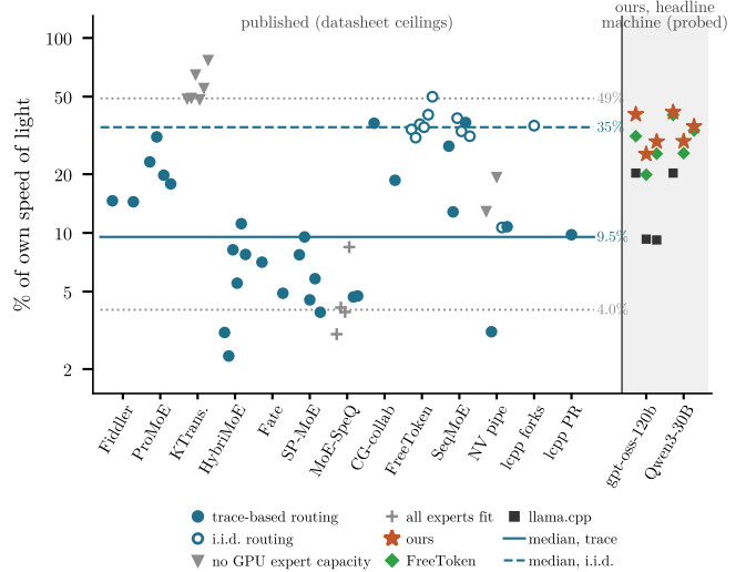
Figure 5: Published MoE-offloading measurements (52 rows from 13 sources) as a percentage of their own speed of light, computed from the paper’s hardware at datasheet rates and, where a routing trace of the model exists, the per-layer Belady optimum (filled); hollow points assume uniform routing, which overstates the optimum’s reads and so the percentage. Right: our cache, FreeToken and stock llama.cpp on listing B against the probed limit of Table 1.
