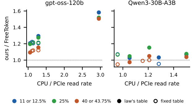
Figure 4: Ours over FreeToken’s better backend (carried over from listing B for job 089) in every same-machine comparison of the current engine on the two models of Table 1 (jobs 076–089, eight hosts), against the machine’s CPU-to-PCIe read ratio (FreeToken’s own probe). Filled: FETCH table from the law on that machine; hollow: the fixed table. The rightmost gpt-oss points are the Core i9-14900K with FreeToken’s executor on its performance cores (job 088; the confounded job 085 points are omitted); the rightmost Qwen3 points are the Ryzen 9 7900; the points at 1.05 are the second-host rerun of Table 1 (job 089).
