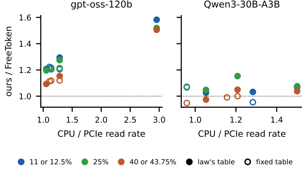
Figure 2: Ours over FreeToken’s better backend (carried over from host B on host S) in every same-machine comparison of the current engine on the two models of Table 3paper.pdf (eight machines), against the machine’s CPU-to-PCIe read ratio (FreeToken’s own probe). Filled: FETCH table from the model on that machine; hollow: the fixed table. The rightmost gpt-oss points are a Core i9-14900K with FreeToken’s executor on its performance cores; the rightmost Qwen3 points are a Ryzen 9 7900.
