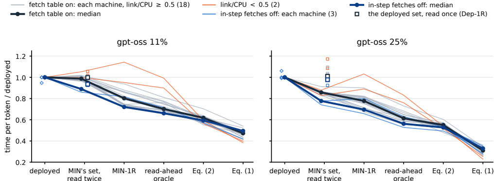
Figure 2. Where the seconds go, measured: each state's time per token relative to the deployed cache on the same machine (lower is faster) as what is cached changes (MIN's set, read twice; squares: the deployed set, read once), then both, then when, with the two bounds. One line per machine. Grey (orange: link-to-CPU ratio below 0.5): the deployed read path, where the second state is MIN's schedule with the fetch table, not its set held. Blue: in-step fetches off (diamonds: the deployed cache without them). Thick: medians over fast-link machines.
