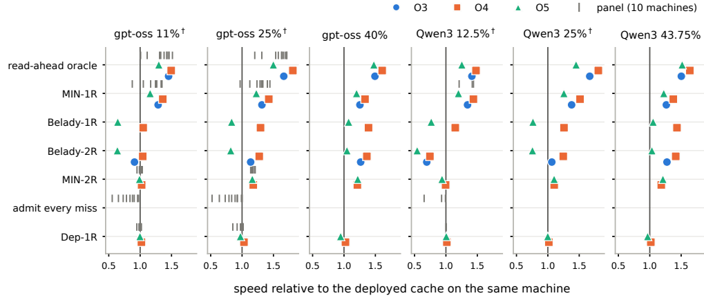
Figure 3. What foresight is worth, by how it is spent: speed of each configuration of Table 2 relative to the deployed cache on the same machine, at the six budgets ( \dagger host-bound). Three machines at every budget (O3–O5: two Ryzen 9 9950X and a 9950X3D); the 10 machines of the panel’s main job (grey ticks) at the two host-bound gpt-oss budgets, and 3 of them at Qwen3 12.5%. The 95% intervals are mostly narrower than the markers. MIN-1R gains at every budget on these machines; reading twice or admitting what MIN bypasses gains at some budgets and loses at others.
