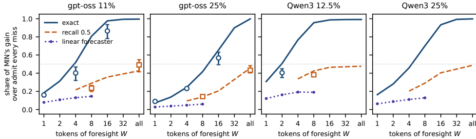
Figure 5. Baseline here: admit every miss , not the deployed cache. The share of MIN’s gain over admitting every miss recovered, in host reads on the routing the engine runs, by exact routing of the next W tokens (solid), by a window whose experts are each right with probability 0.5 (dashed) and by a linear forecaster fitted on other text (dotted). Markers: the same share in time per token (mean and range over the panel’s main-job machines: 10 for gpt-oss, 3 for Qwen3 12.5%). Grey line: half of the gain.
