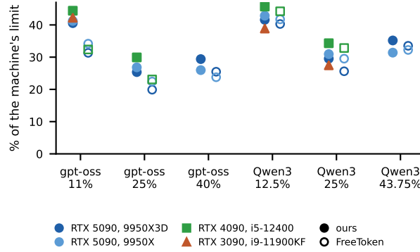
Figure 5. Ours (filled) and FreeToken (hollow) as a percentage of each machine’s own bound (exact optimum, the machine’s highest probed host rate, the card’s datasheet rate) at every cell of Table 7: two RTX 5090 hosts, an RTX 4090 and an RTX 3090 (FreeToken’s 3090 cells, its carried-over backend running below llama.cpp, are omitted). The limit ranges from 41 to 519 tok/s across these cells; ours stays at 25–46% of it.
