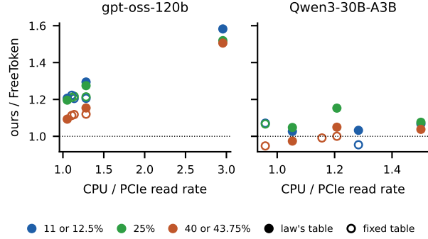
Figure 6. Ours over FreeToken’s better backend (carried over from host B on host S) in every same-machine comparison of the current engine on the two models of Table 2 (eight hosts), against the machine’s CPU-to-PCIe read ratio (FreeToken’s own probe). Filled: FETCH table from the model on that machine; hollow: the fixed table. The rightmost gpt-oss points are a Core i9-14900K with FreeToken’s executor on its performance cores; the rightmost Qwen3 points are a Ryzen 9 7900.
