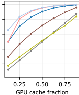
gpt-oss-20b (E=32, k=4)
