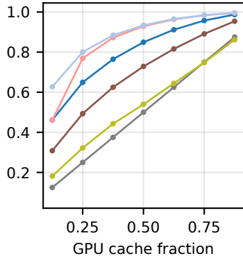
olmoe-1b-7b (E=64, k=8)
