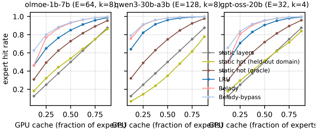
Figure 2: Expert hit rate against GPU cache size (as a fraction of each layer’s experts) for static and dynamic policies.
