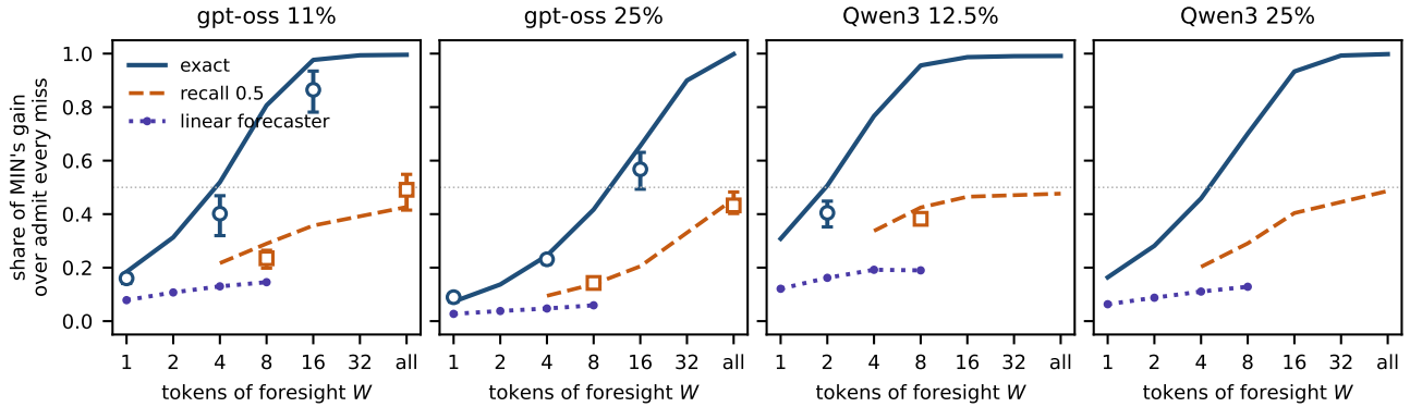
Figure 5. Baseline here: admit every miss , not the deployed cache. The value of partial foresight at the four host-bound budgets: the share of MIN’s gain over admitting every miss recovered by exact routing of the next W tokens (solid), by a window whose experts are each right with probability 0.5 (dashed), and by a linear forecaster fitted on other text (dotted), in host reads on the routing the engine runs. Markers: the same share in time per token on the panel machines (mean and range over machines; 10 machines for gpt-oss, 3 for Qwen3 at 12.5%). The grey line marks half of the gain.
