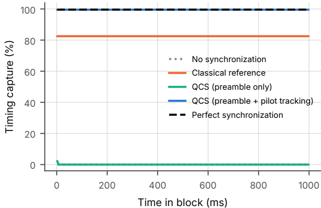
(a) 25 km, oscillator wander 0.2 ppm/ \sqrt{\text{ms}}
