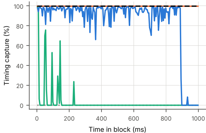
(b) 125 km, oscillator wander 0.2 ppm/ \sqrt{\text{ms}}
