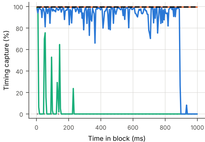
(b) 125 km, oscillator wander 0.2 ppm/ \sqrt{\text{ms}}
