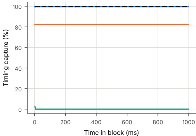
(a) 25 km, oscillator wander 0.2 ppm/ \sqrt{\text{ms}}
