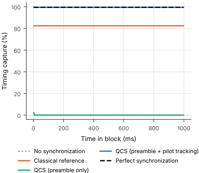
(a) 25 km, oscillator wander 0.2 ppm/ \sqrt{\text{ms}}
