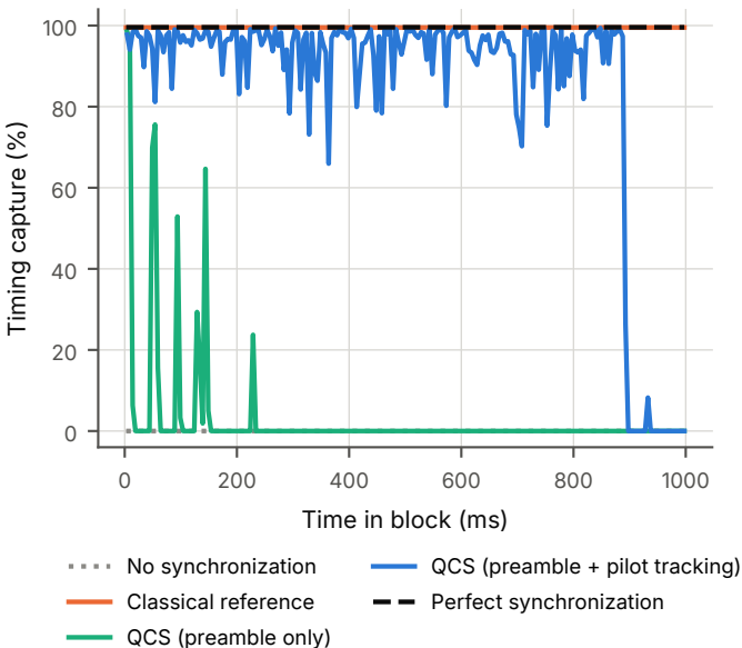
(b) 125 km, oscillator wander 0.2 ppm/ \sqrt{\text{ms}}
