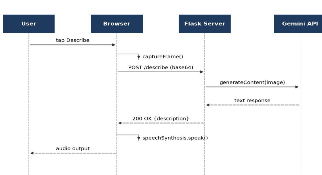
Fig. 4.3 Sequence Diagram – /describe Request
