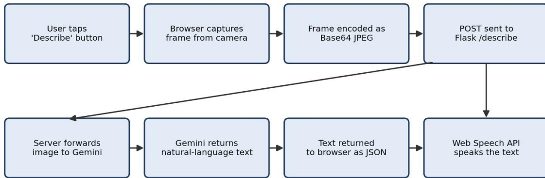
Fig. 3.1 End-to-End System Workflow
