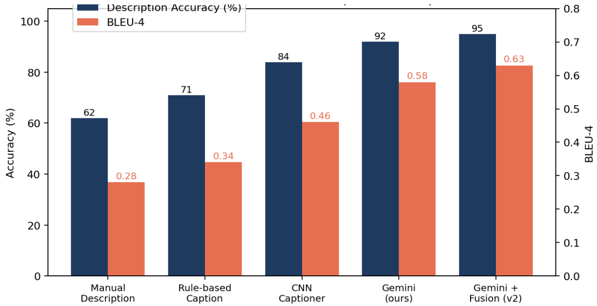
Fig. 6.1 Comparative Performance of Caption / Description Methods
