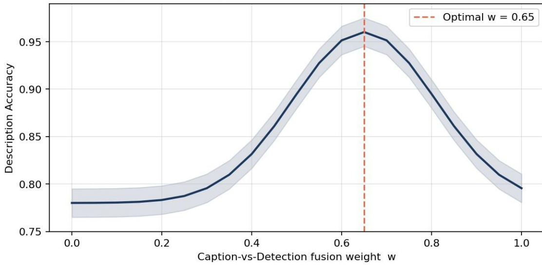
Fig. 5.2 Sensitivity of Description Accuracy to Fusion Weight
