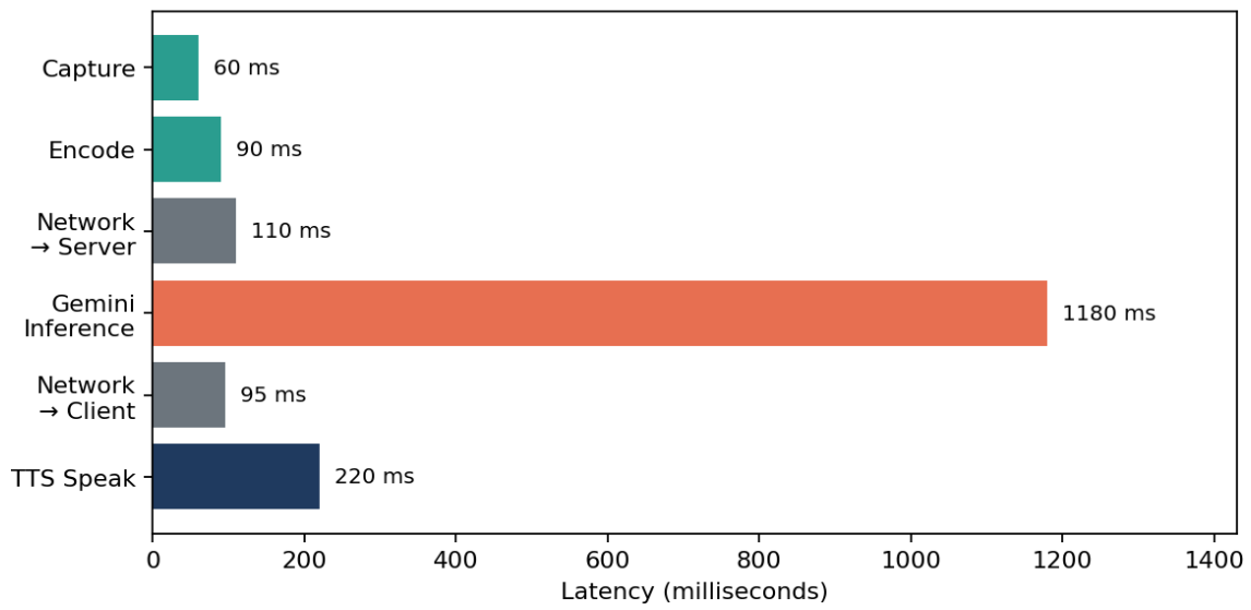
Fig. 6.2 End-to-End Latency Breakdown (mean of 50 runs)
