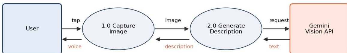
Fig. 4.2 Data-Flow Diagram (Level-1)
