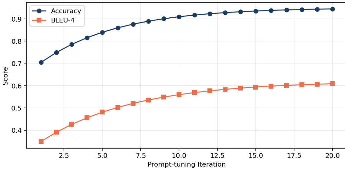
Fig. 6.4 Improvement of Output Quality over Prompt-Tuning Iterations
