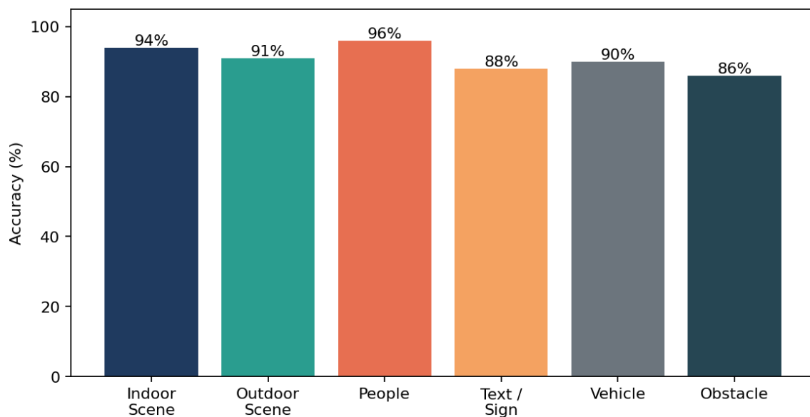
Fig. 6.3 Per-Category Description Accuracy
