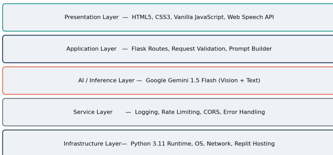
Fig. 4.1 Layered View of the AI Vision System
