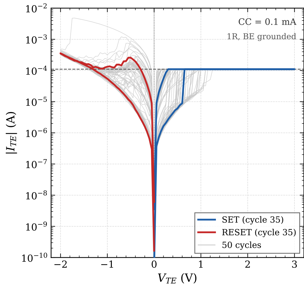
Bipolar I-V (SET/RESET)
