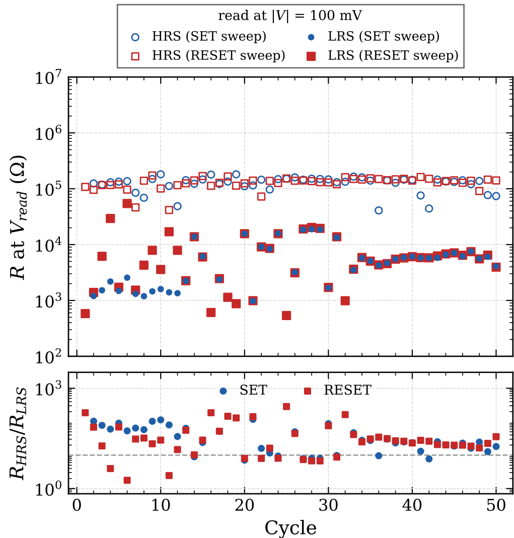
Endurance / Window (SET: 25 \times , RESET: 26 \times )
